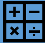
Math
